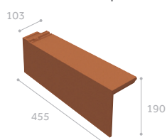
Topo de remate angular
